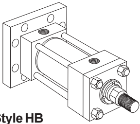
Style HB Cap Square Flange (NFA Style MF6)
