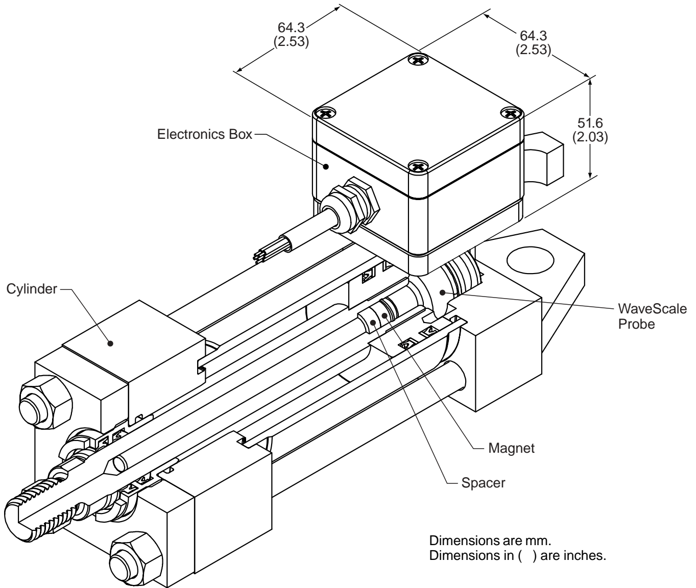
Cutaway View
