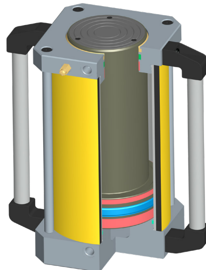
Lightraulics® Heavy Duty Tie Rod Cylinder ▶ with 50 bar retraction pressure Available capacities: 50t - 410t
