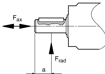
Fig. 1: Loading on output shaft.
