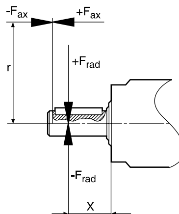
Fig 2: Load and braking torque on output shaft of planetary gear
